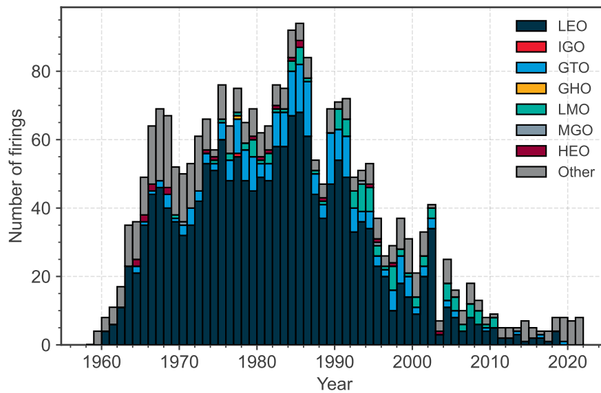
Figure 4.5: Evolution solid rocket motor firings by orbit type.
