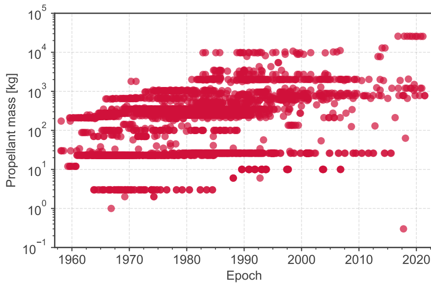
Figure 4.4: Evolution solid rocket motor firings.
