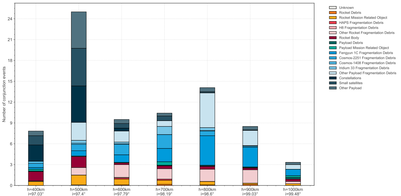
Figure 3.11: Conjunction events, and chaser classification, for a set of representative targets in Sun-synchronous orbits over 2021.
