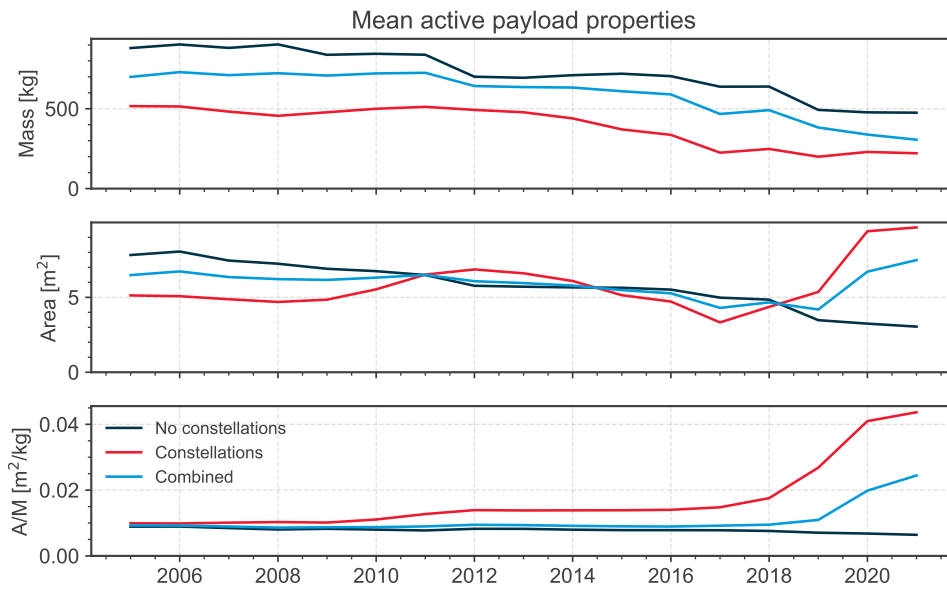
Figure 2.25: Payload parameters for active payloads in LEO over time.
