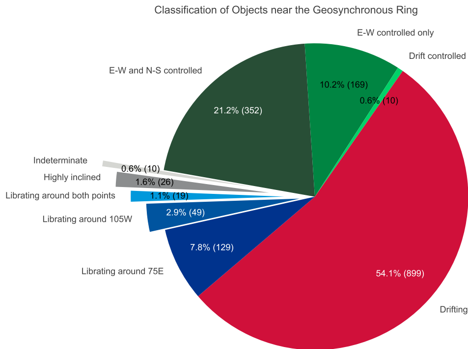
Figure 6.18: Orbital evolution status of payloads near the Geostationary orbit during 2021.
