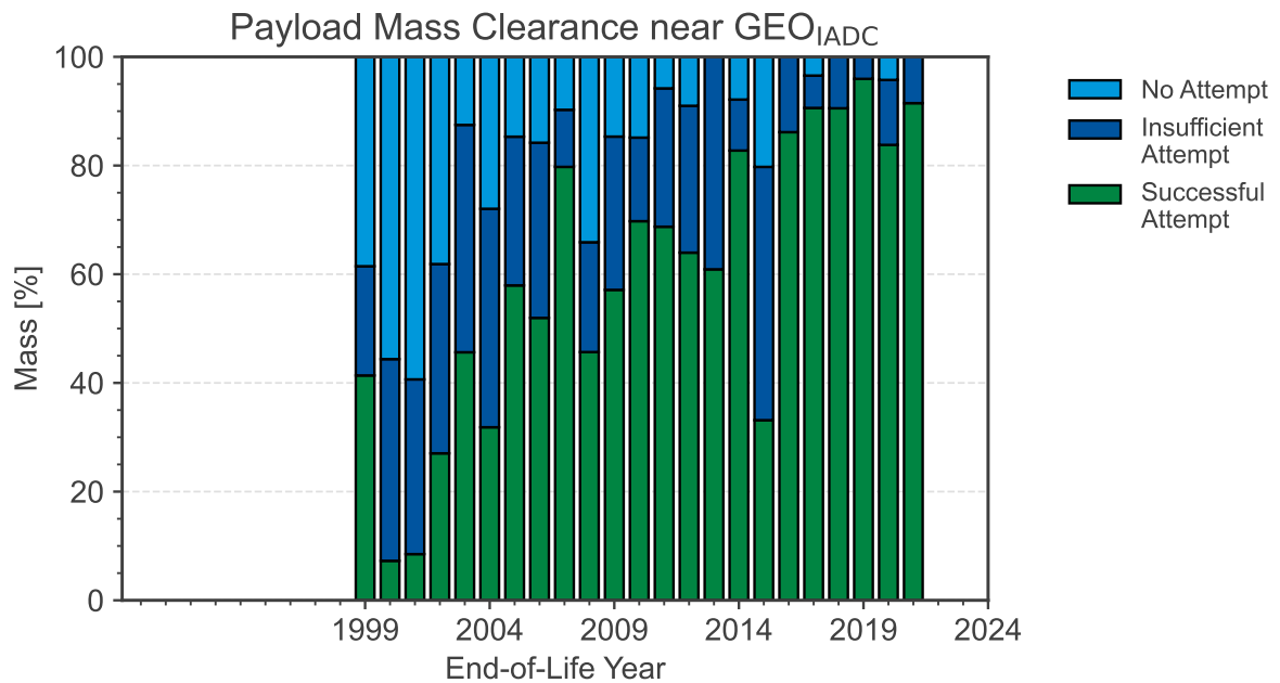
(b) Relative mass clearance near GEO IADC .
