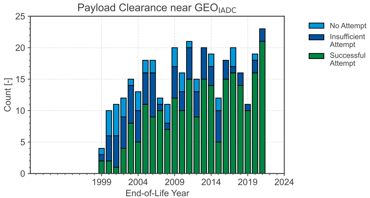
(a) Absolute clearance near GEO IADC .
