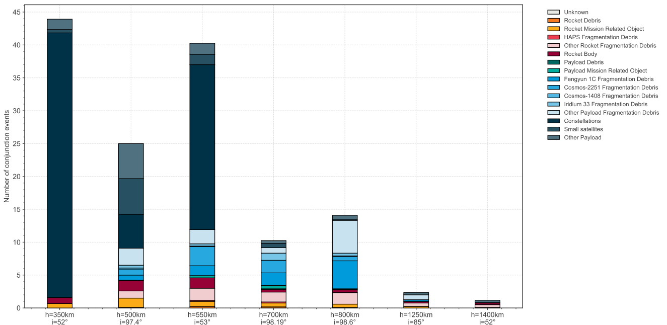
Figure 4: Conjunction events (i.e. events that could trigger an operator response but not necessarily an avoidance manoeuvre nor a collision) and corresponding chaser classification for a set of representative missions over 2021.
