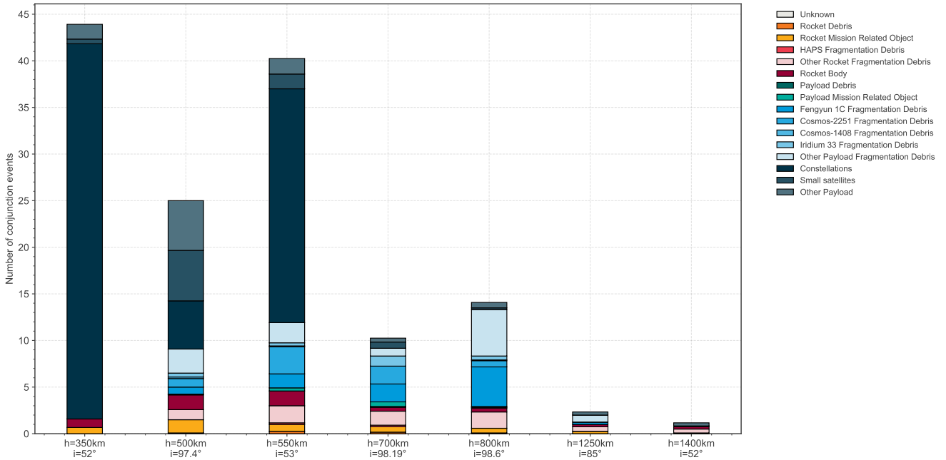
Figure 3.10: Conjunction events, and corresponding chaser classification, for a set of representative targets over 2021.
