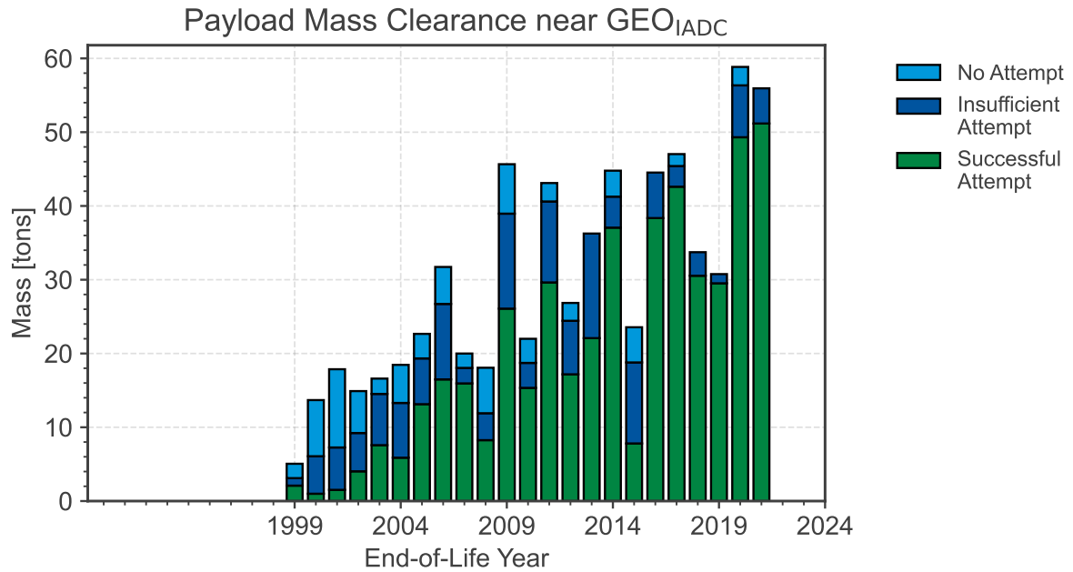
(a) Absolute mass clearance near GEO IADC .
