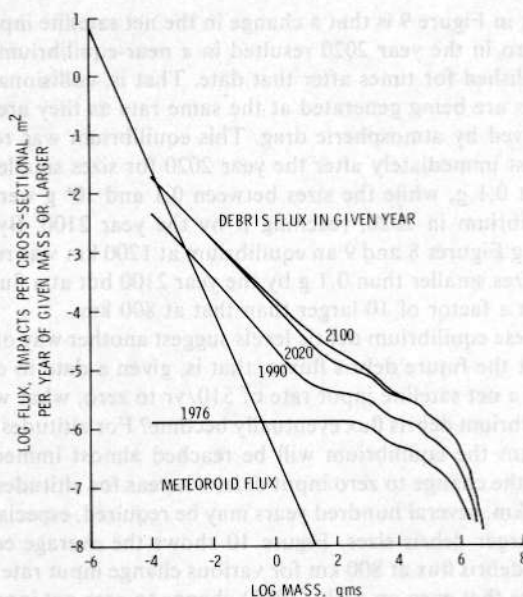
Fig. 9. Average debris flux at 800 km; assumes that the net satellite input rate changes from 510/yr to zero in the year 2020.
