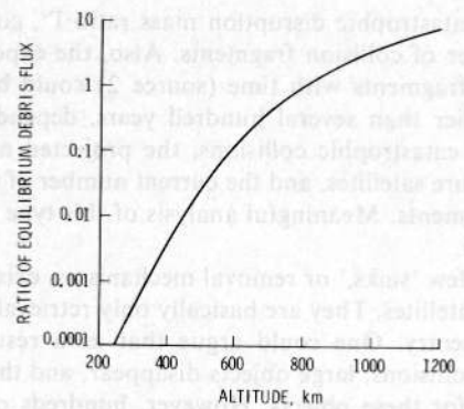
Fig. 11. Ratio of equilibrium debris flux at given altitude to flux at 800 km.
